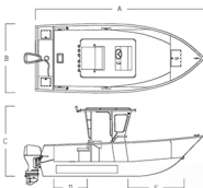
Line-Drawing-K-V-211-Hardtop
